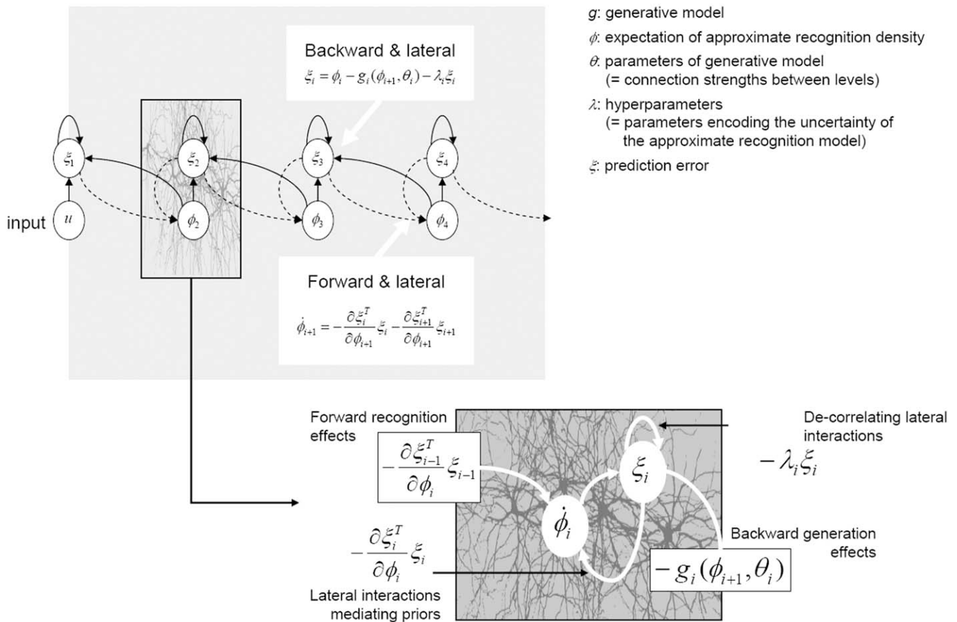
Figure 2. Upper panel: Schematic of a hierarchical neural architecture for implementing predictive coding. Each level in this model provides predictions (priors) to representations in the level below. The upper circles represent neural units encoding prediction error ( \xi ) and the lower circles represent neural units encoding the conditional expectation of causes ( \phi ). At all levels, these expectations change to minimize the prediction error, i.e., the discrepancy between the prediction from the level above and the input from the level below. These two constraints correspond to prior and likelihood terms, respectively (see main text). Lower panel: Details of the influences on representational and error units at a single level in the hierarchy. See Friston (2003, 2005a) for details.
